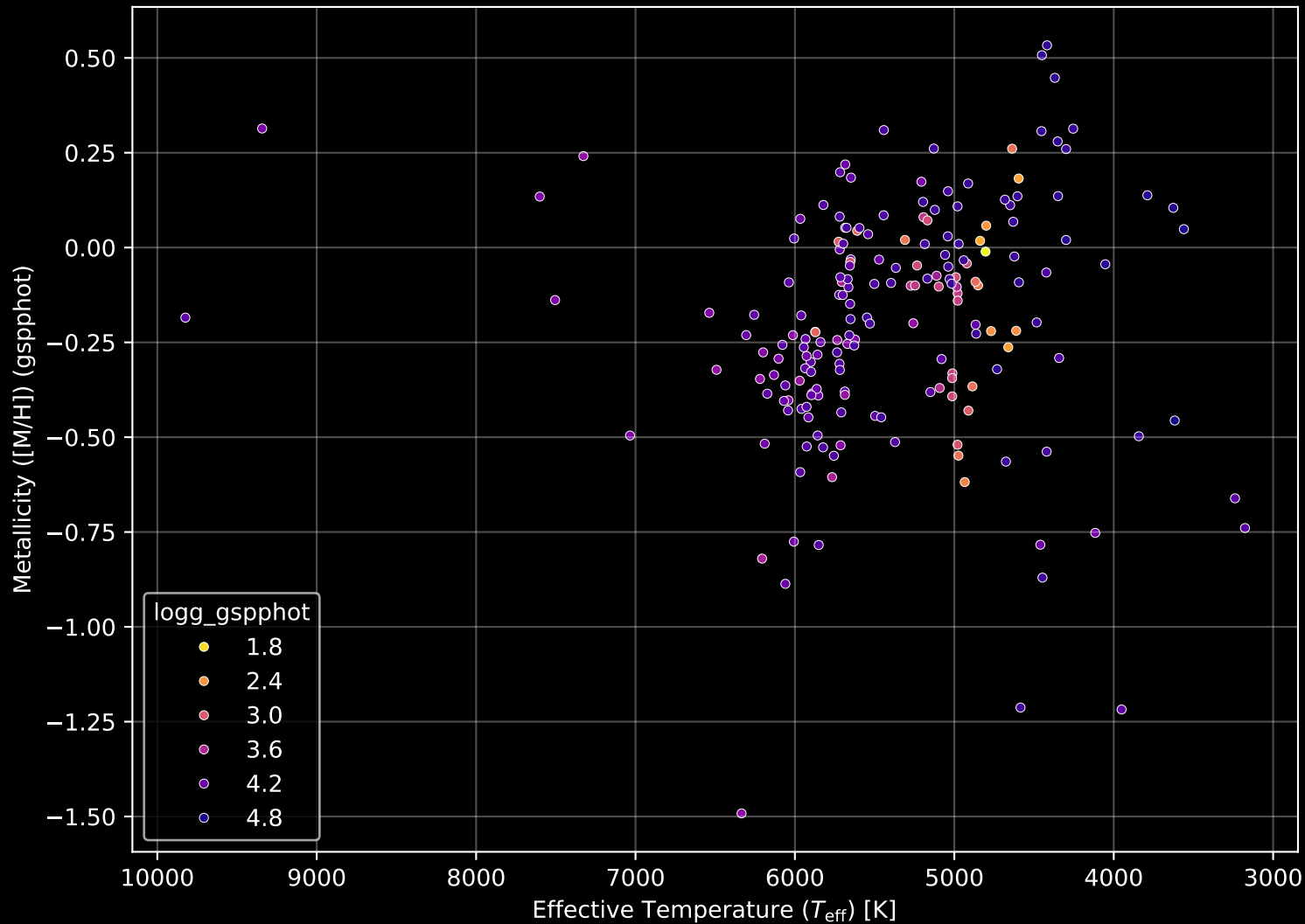
APOGEE DR17 Field: [160+56_MGA] Stellar Population Parameters (n= 189)
