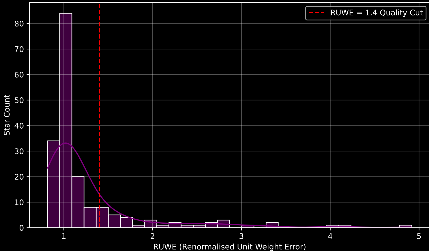
GAPOGEE DR17 Field [160+56_MGA] RUWE Distribution (n= 183)
