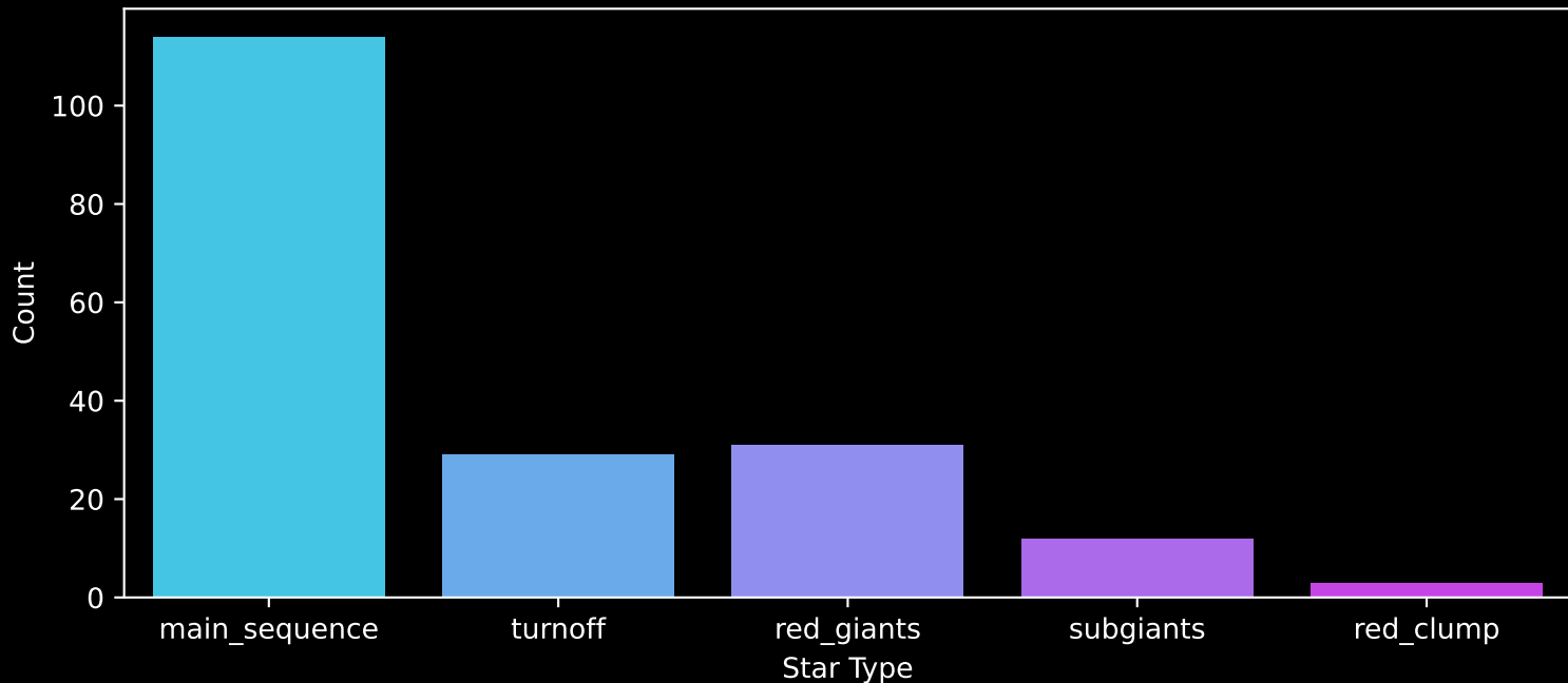
APOGEE DR17 Field: [160+56_MGA] Count plot of Star Type
