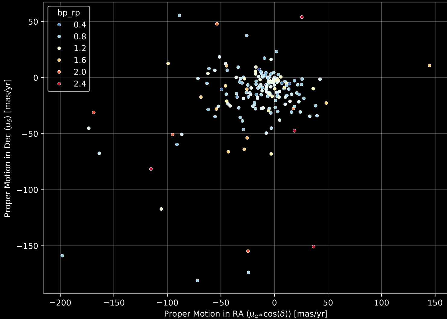
APOGEE DR17 Field: [160+56_MGA] Proper Motion Diagram (n= 189)
