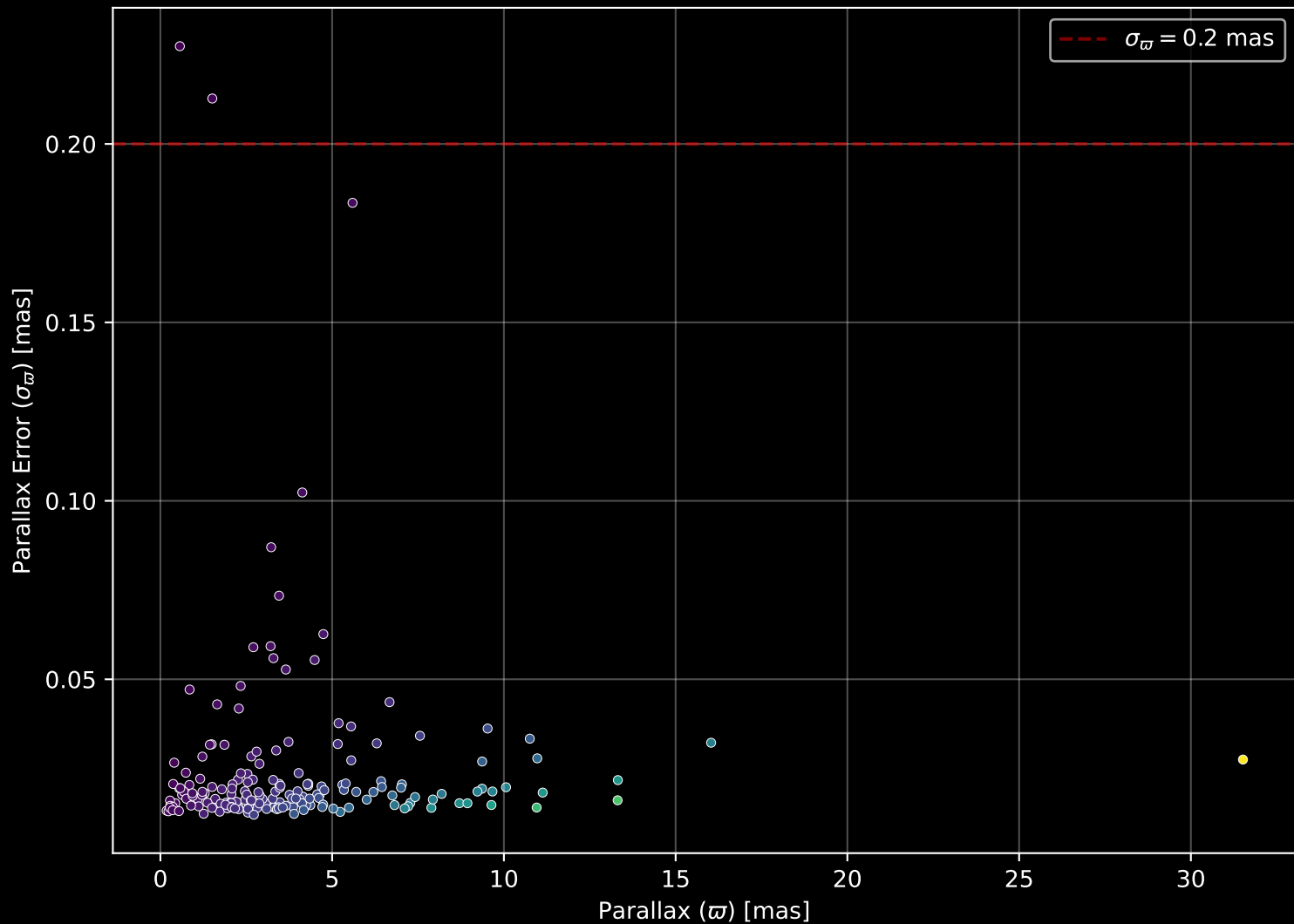
APOGEE DR17 Field: [160+56_MGA] Parallax Quality (n= 189)
