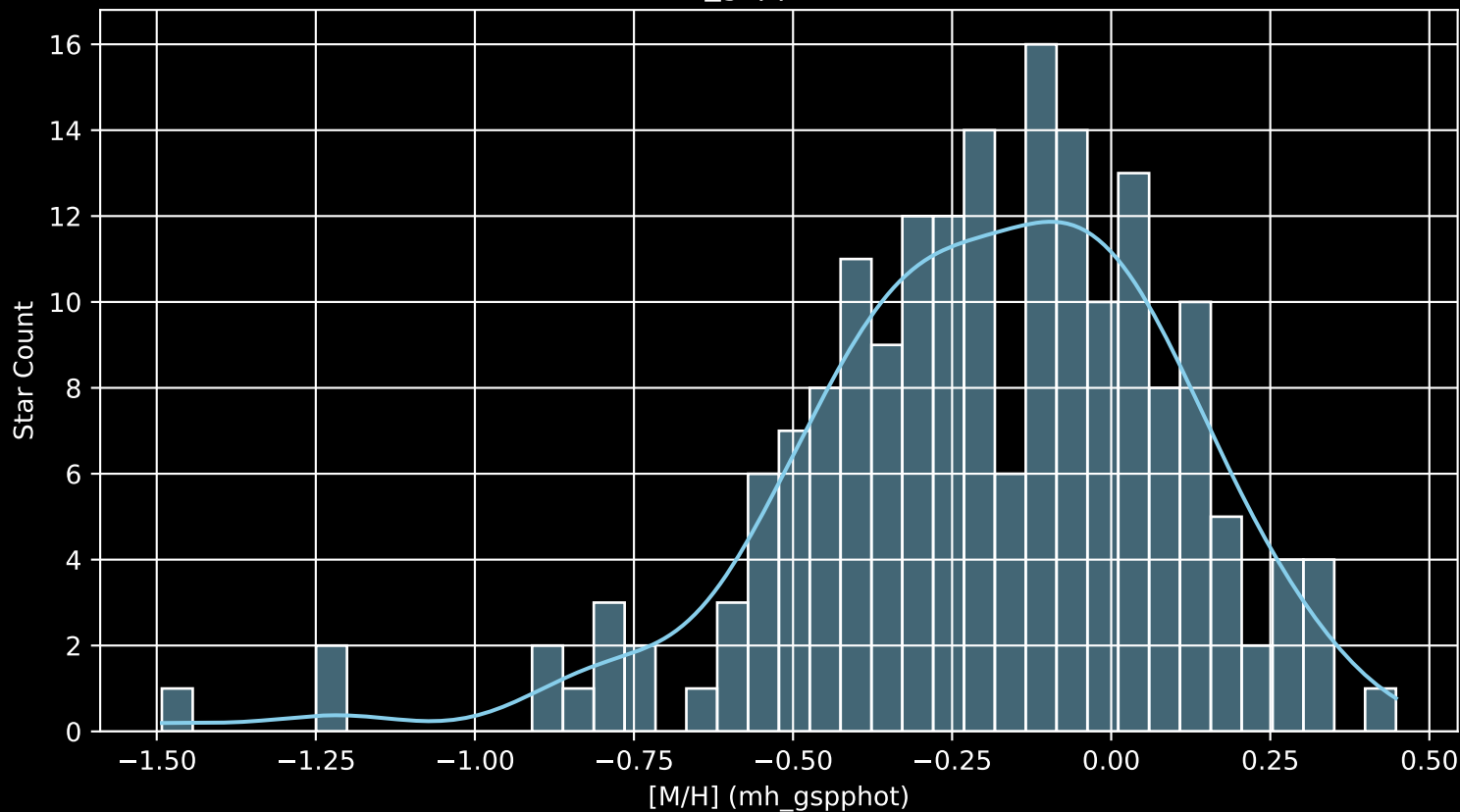
APOGEE DR17 Field: [160+56_MGA [M/H] (mh_gspphot) (n= 187)
